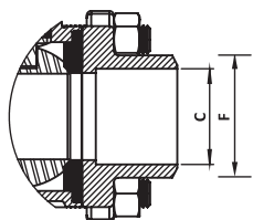
Butt Weld Ends
